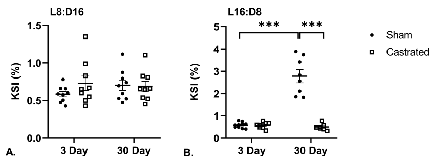
Fig. 2. Kidney somatic index (KSI) of sham-operated and castrated fish under short day (L8:D16, A.) or long day (L16:D8, B.) photoperiod (N = 10 in each group, means \pm SE shown, *** p < 0.001 ).
