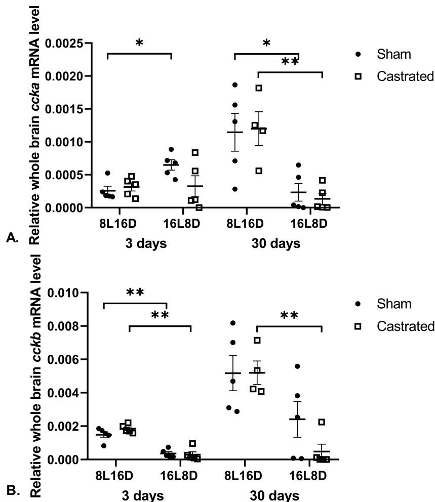
Fig. 4. Whole brain ccka (A) and cckb (B) mRNA levels in the stickleback males under short day (L8:D16) or long day (L16:D8) photoperiod for 3 days or 30 days ( N = 5 in each group, means \pm SE shown, *p < 0.05 ; **p < 0.01 ).
