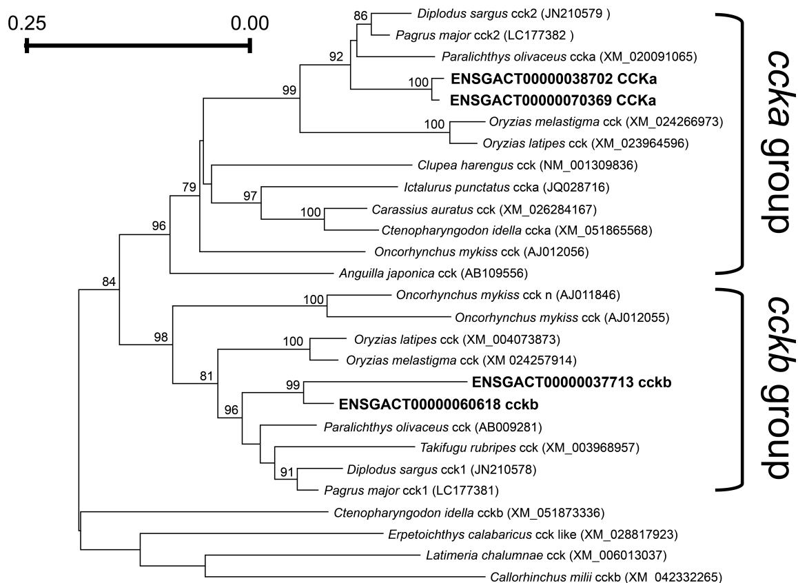
Fig. 3. Neighbor-joining (NJ) tree of fish cck gene inferred from dataset comprising 858 aligned base pairs with 10,000 bootstrap replicates. Each terminal node is marked with the scientific name, followed by the gene definition, and the GenBank accession. The four three-spined stickleback cck transcript variants are shown in bold. Only nodes with bootstrap values of 70 or higher are labeled.
